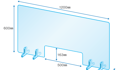
NCW-4 (W1200mm×H600mm)
